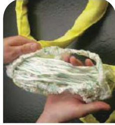
Sling Overload Failure
