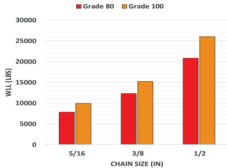
WLL of Slings
