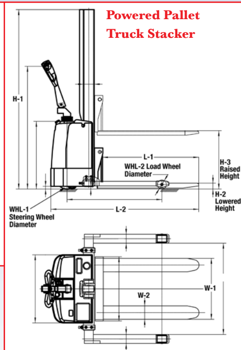
Powered Pallet Truck Stacker
